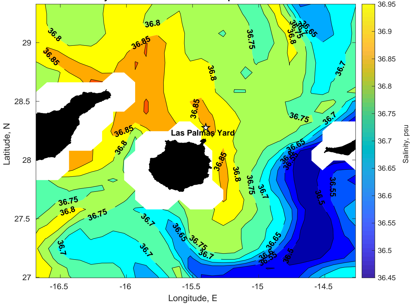
Surface Salinity for Las Palmas Yard at 28-Apr-2024 00:00:00
